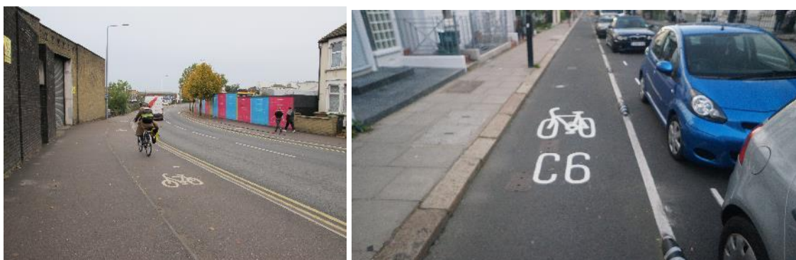
Figure 6-9: Blackhorse Lane (left) has installed narrow cycle tracks alongside the existing footway with a small kerb upstand, and Cycleway 6 (right) has used light segregation to provide cycle tracks in narrower sections of the route
